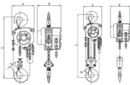
KT-C Chain Block (Single Chain)
